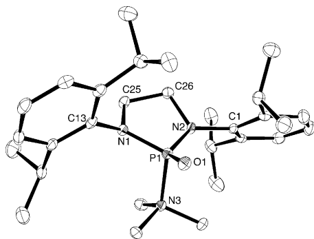
Figure 1. Solid-state structure of [2]^+ (hydrogen atoms and the [\text{GaCl}_4] anion have been omitted for clarity). Ellipsoids are projected at 50% probability. Selected bond lengths [Å] and angles [°]: N1–P1 1.6306(18), N2–P1 1.6345(19), N3–P1 1.8431(19), O1–P1 1.4586(15), C25–N1 1.488(3), C25–C26 1.527(3), C26–N2 1.490(3); C13–N1–C25 119.36(17), C13–N1–P1 123.99(15), C25–N1–P1 111.58(14), C1–N2–C26 116.48(17), C1–N2–P1 129.53(15), C26–N2–P1 111.02(14), O1–P1–N1 119.61(9), O1–P1–N2 124.70(9), N1–P1–N2 97.50(9), O1–P1–N3 101.22(9), N1–P1–N3 107.09(9), N2–P1–N3 105.23(9).
